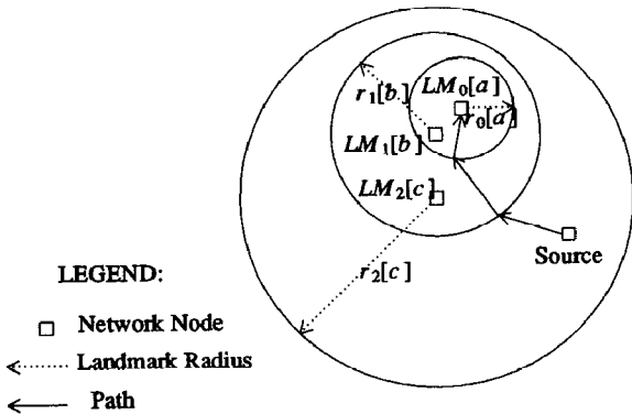
Figure 3: Landmark Hierarchy
